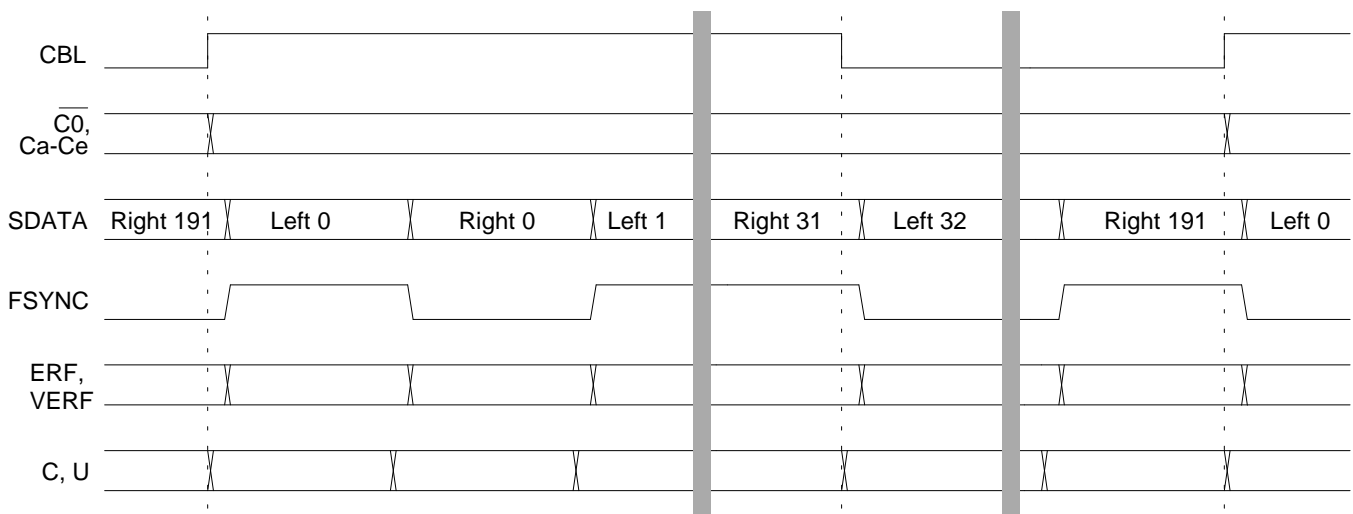
Figure 19. CBL Timing
